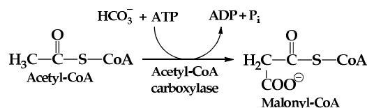
Fig. 2. Acetyl CoA carboxylase catalyzed reaction; the first step in the sequence of reactions for the biosynthesis of fatty acids [25]
