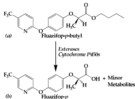
Fig. 1. Metabolism of fluazifop-p-butyl (a) to fluazifop-p (b) and other minor metabolites [17]
