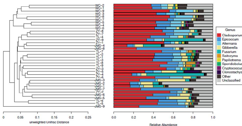
Fig. 5. Unweighted pair-group method with arithmetic means (UPGMA) analysis of microbial community structure based on ITS gene amplicon sequencing data
